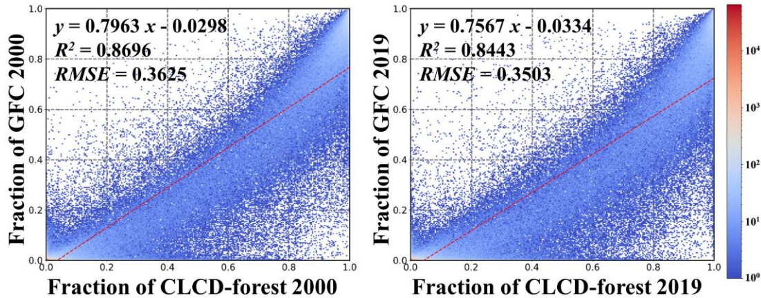
Figure 8. Scatterplots of forest fraction between the CLCD and GFC in 2000 and 2019. Forest fraction was aggregated within the 0.05^\circ by 0.05^\circ spatial grid.
