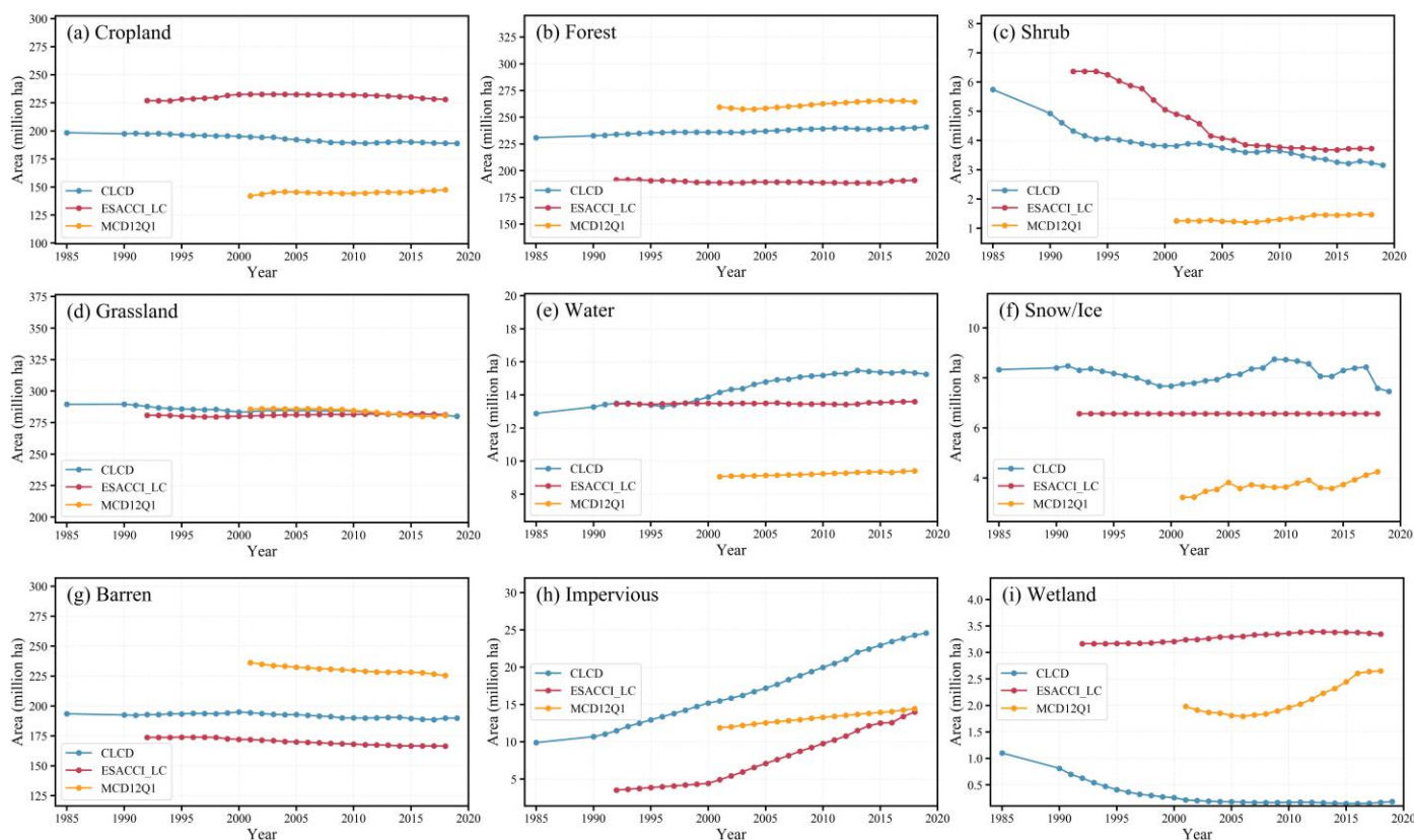
370 Figure 12. Temporal changes in area of different land covers in China from 1985 to 2019.
