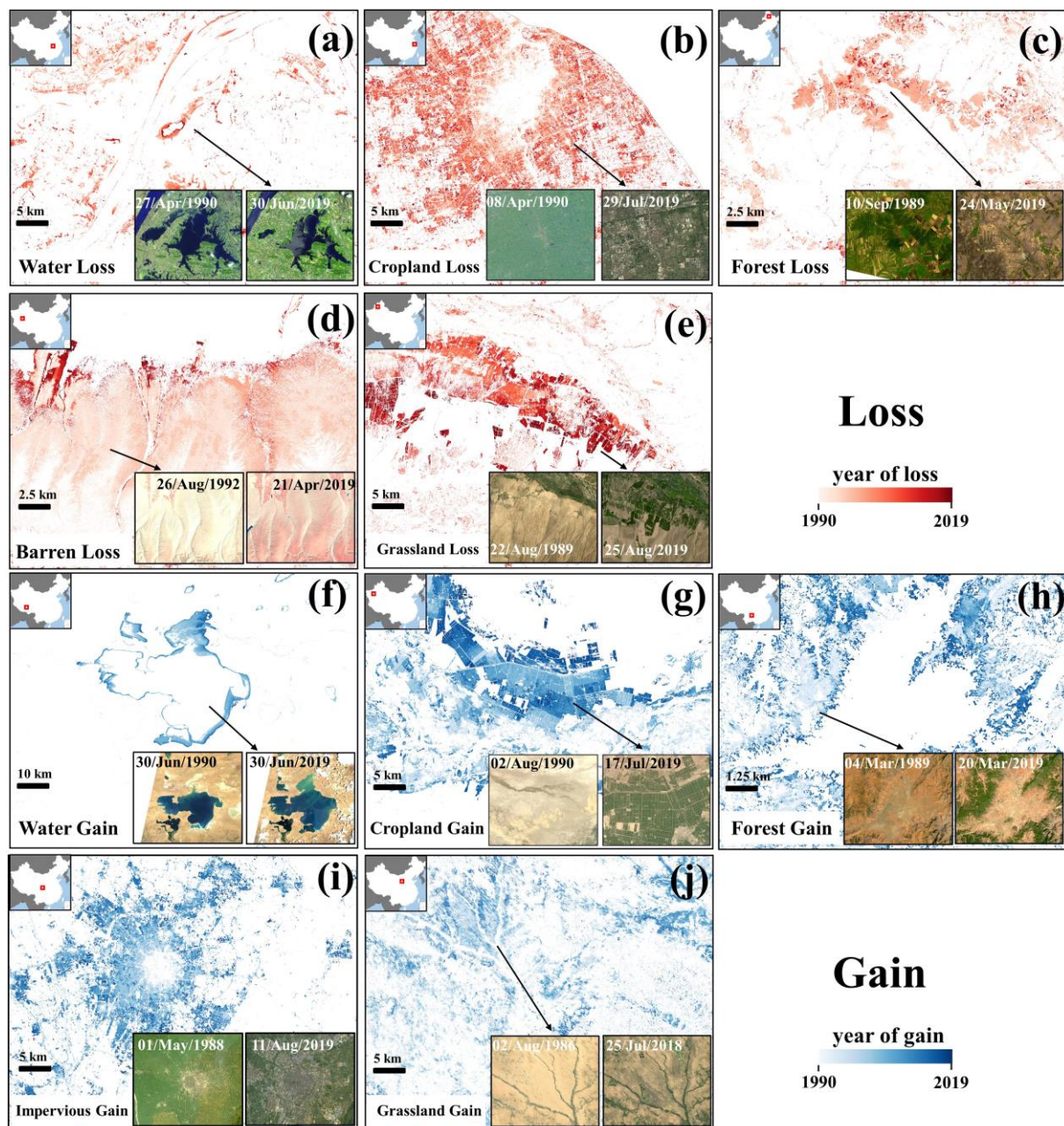
395 Figure 13. Typical land cover changes and conversions observed in China from 1985 to 2019: (a) lake shrinkage in Wuhan City (30.543703° N, 114.296992° E); (b) cropland loss due to the urbanization in Shanghai City (31.214542° N, 121.490796° E); (c) deforestation induced by reclamation in northeast China (49.508726° N, 124.939498° E); (d) bare land converted to grassland in the Qira oasis, located at the southern fringe of the TAKLAMAKAN Desert (36.237807° N, 81.215592° E). The illustration is of Landsat images with false-colour combination (R: NIR, G: Red, B: Green) to enhance the grassland; (e) grassland loss due to the 400 reclamation in northwest China (43.575843° N, 80.987817° E); (f) Siling Co Lake expansion in the Tibet Plateau (31.793826° N, 89.057216° E); (g) reclamation in the Aksu Prefecture (40.593062° N, 81.048109° E); (h) afforestation in Yunnan Province (26.518645° N, 103.613297° E); (i) Expansion of Chengdu City (30.666955° N, 104.068452° E); (j) grassland gain in the Mu Us Desert, Yulin City (38.509526° N, 109.660052° E).
