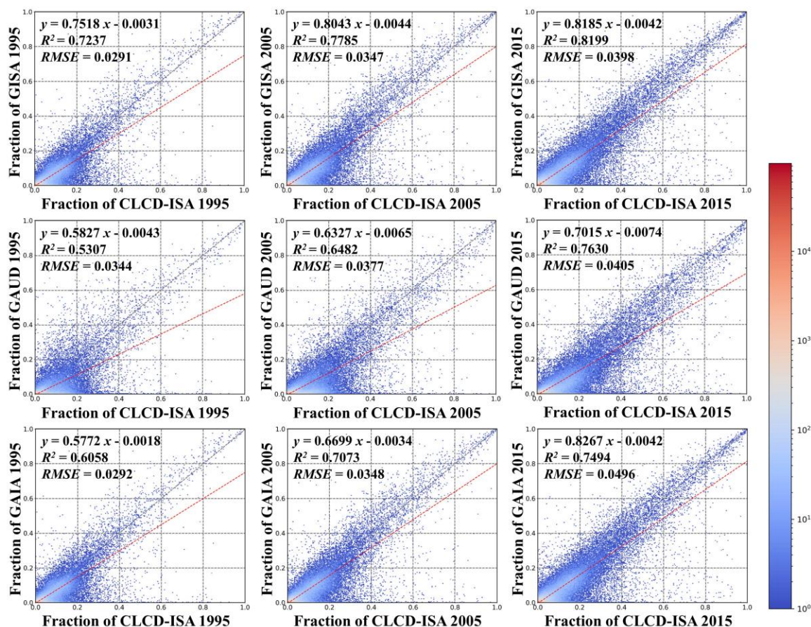
290 Figure 6. Scatterplots of ISA fraction between different products in 1995, 2005 and 2015, respectively. ISA fraction was aggregated within the 0.05° by 0.05° spatial grid.
