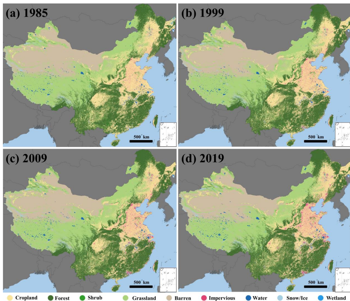
250 Figure 4. Annual China Land Cover Dataset (CLCD) for 1985, 1999, 2009 and 2019.
