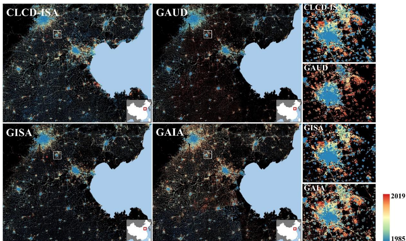
305 Figure 7. Comparison between different ISA products over North China Plain, with zoom-in maps located in Langfang City ( 39.526545^{\circ} N, 116.703692^{\circ} E).
