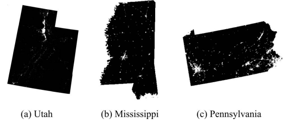
Fig. 3. Results produced by the proposed method in the three selected states of the U.S.
