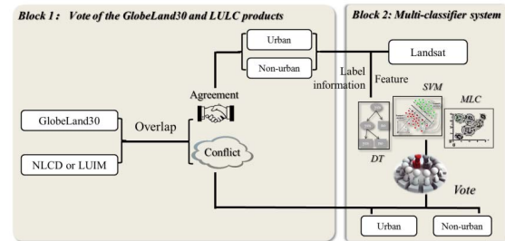
Fig. 1. Proposed urban area delineation method integrating multisource data.
