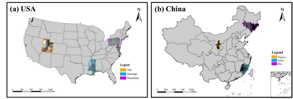
Fig. 2. Study areas. (a) Three selected states in the U.S. as well as their 2010 Landsat images. (b) Three selected provinces in China as well as their 2010 Landsat images.
