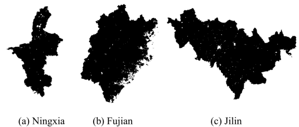
Fig. 5. Results produced by the proposed method in the three selected provinces of China.
