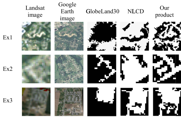
Fig. 4. Some test examples randomly selected from the study areas.
