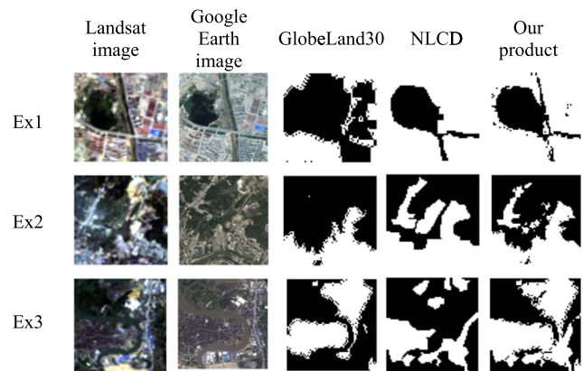
Fig. 6. Some test examples randomly selected from the study areas.
