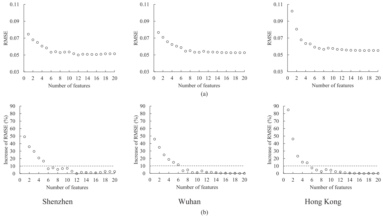
Fig. 12. Accuracy of the estimated building density obtained using feature subsets composed of different numbers of features. (a) RMSE. (b) Percentage increase of RMSE.
