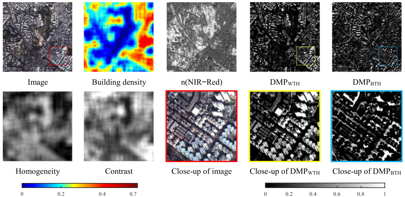
Fig. 2. Example of building density and some representative features for a typical area (see Table I for the complete feature description).
